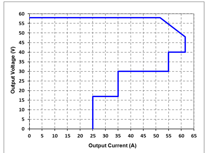
Figure 1 Output feature curve
