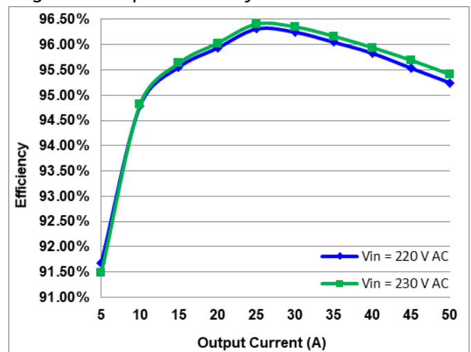
Figure 2 Output efficiency curves
