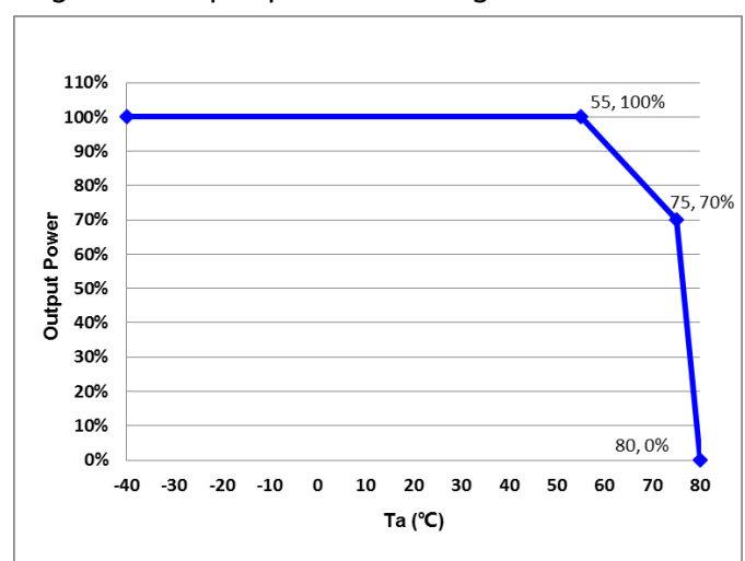
Figure 3 Output power derating curve
